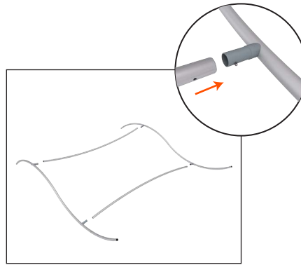
2. Connect center supporting poles.
