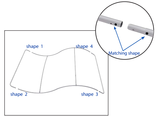
3. Connect corner sections to straight sections with matching shape codes.
